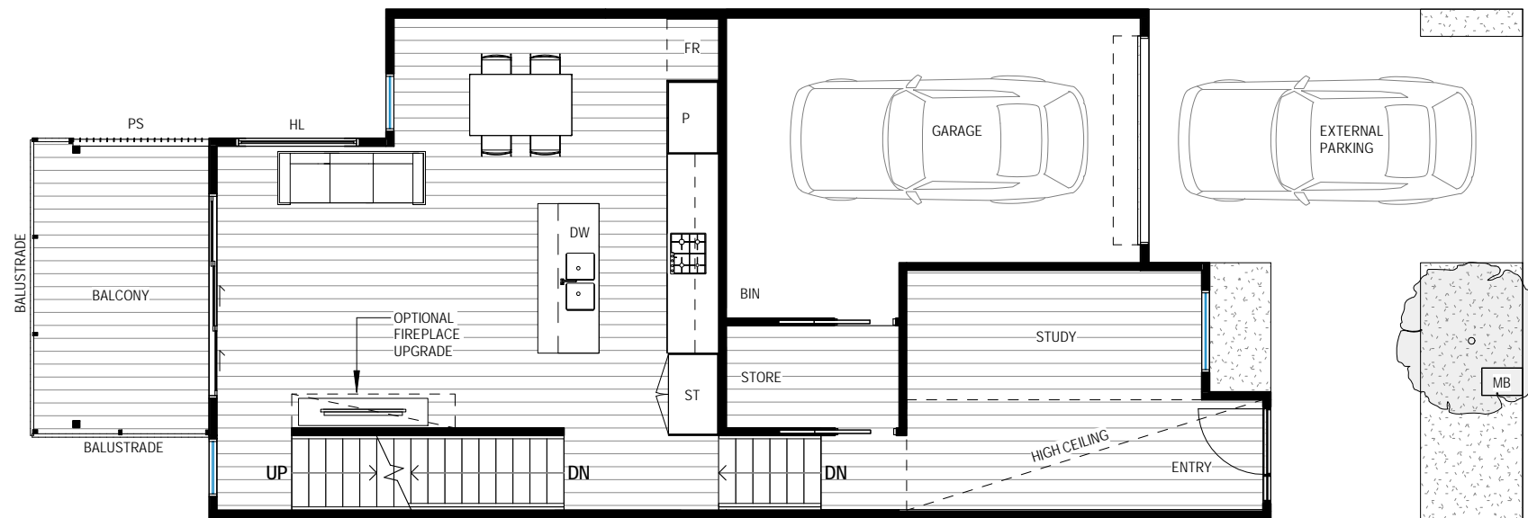
LEVEL 1 FLOOR PLAN
