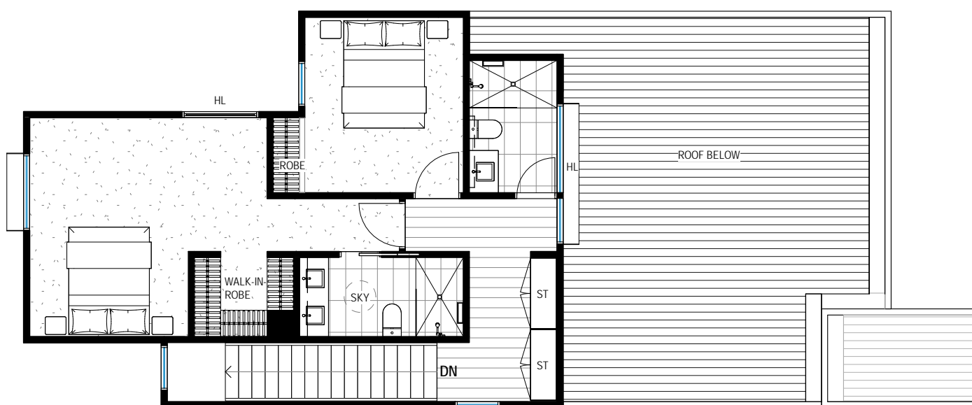
LEVEL 2 FLOOR PLAN
